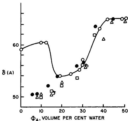
FIGURE 3 Fundamental repeat spacing \delta as a function of the volume per cent water in lecithin-water mesophase. O, this work; \Delta , data from references 5-7; \square , data from reference 8; \bullet , data from reference 9.
