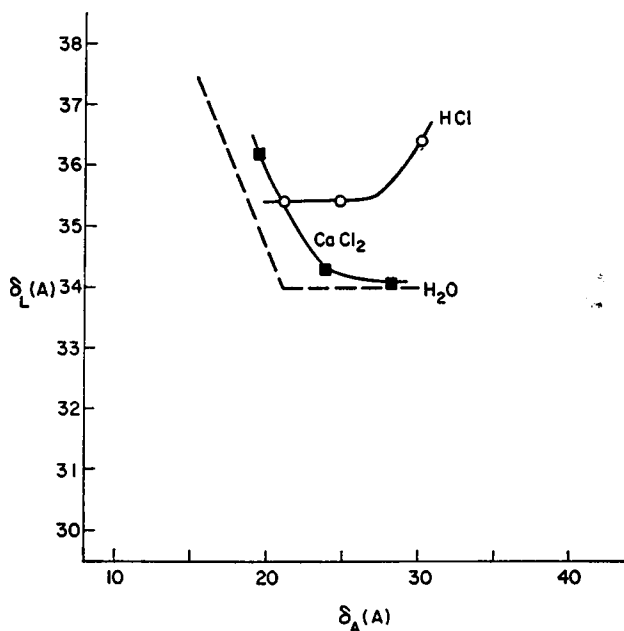
FIGURE 8 Bilayer thickness \delta_L as a function of distance between bilayers \delta_A . ○, HCl solutions; ■, \text{CaCl}_2 solutions.
