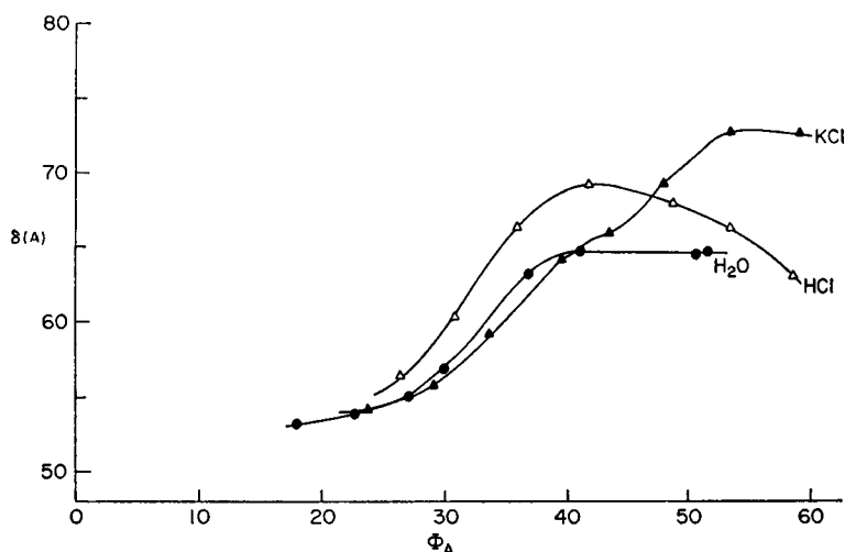
FIGURE 5 Fundamental repeat spacing \delta as a function of volume per cent water or solution in the mesophase. ●, H_2O ; ▲, KCl solutions (1.0 N); △, HCl solutions (1.0 N).
