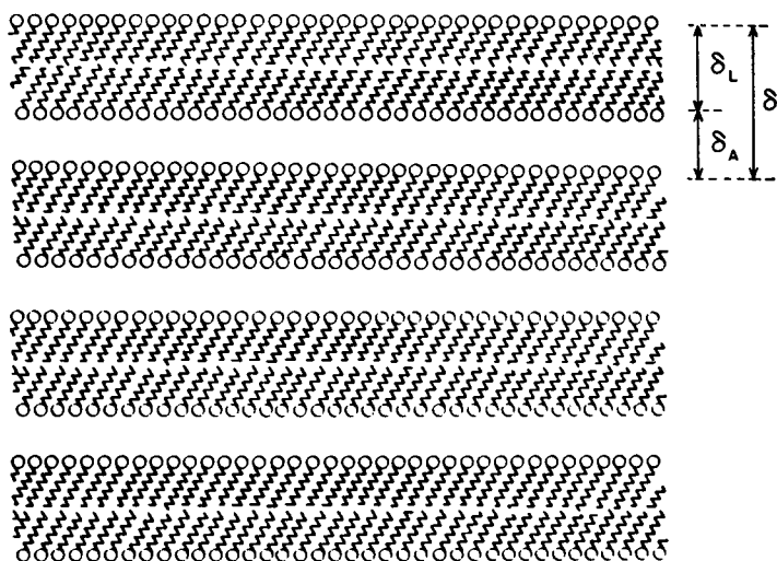
FIGURE 1 Presumed structure for lamellar lipid-water mesophase. \delta = fundamental repeat spacing as obtained from low-angle X-ray diffraction pattern, \delta_L = bilayer thickness, \delta_A = thickness of water layers separating bilayers.
