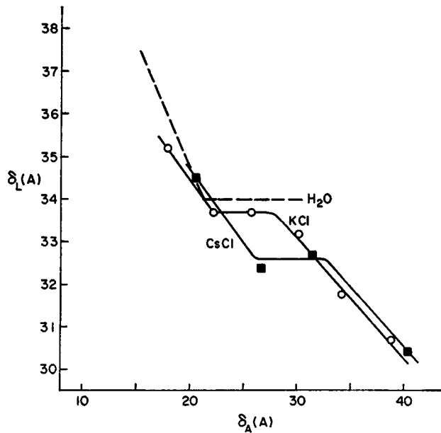
FIGURE 7 Bilayer thickness \delta_L as a function of distance between bilayers \delta_A . ○, KCl solutions; ■, CsCl solutions.
