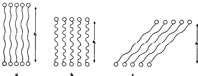
FIGURE 2 Schematic illustration of how changes either in the degree of coiling of the hydrocarbon chains or in their angle of tilt result in changes of bilayer thickness. (a) Relatively uncoiled hydrocarbon chain, perpendicular to plane of bilayer. (b) More highly coiled hydrocarbon chain, perpendicular to plane of bilayer. (c) Relatively uncoiled hydrocarbon chain, tilted with respect to plane of bilayer.
