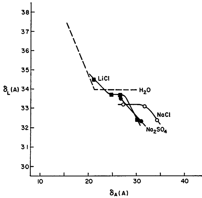
FIGURE 6 Bilayer thickness \delta_L as a function of distance between bilayers \delta_A . ■, LiCl solutions; ○, NaCl solutions; ●, Na 2 SO 4 solutions.
