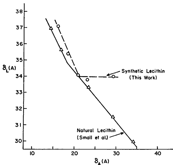
FIGURE 4 Bilayer thickness \delta_L as a function of distance between bilayers \delta_A . O, this work; \Delta , data from references 5-7.
